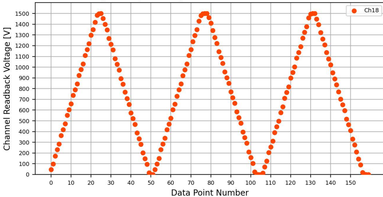
Voltage Ramp Test (Python) Bd #556, Slot #7, Ch #18
