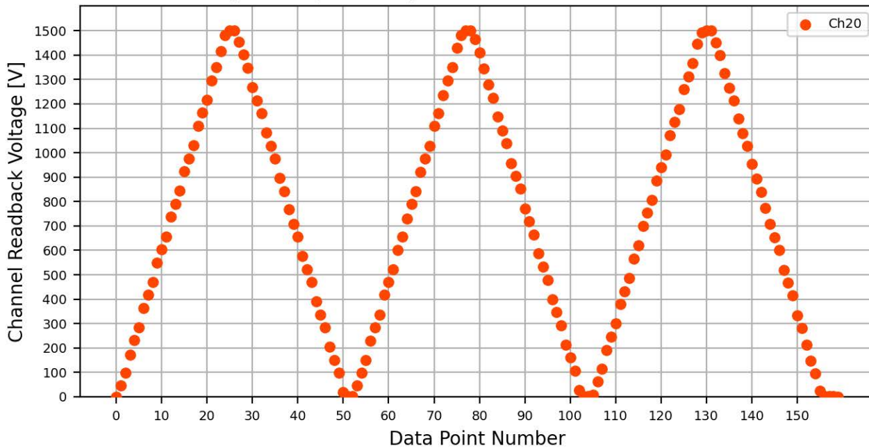
Voltage Ramp Test (Python) Bd #556, Slot #7, Ch #20
