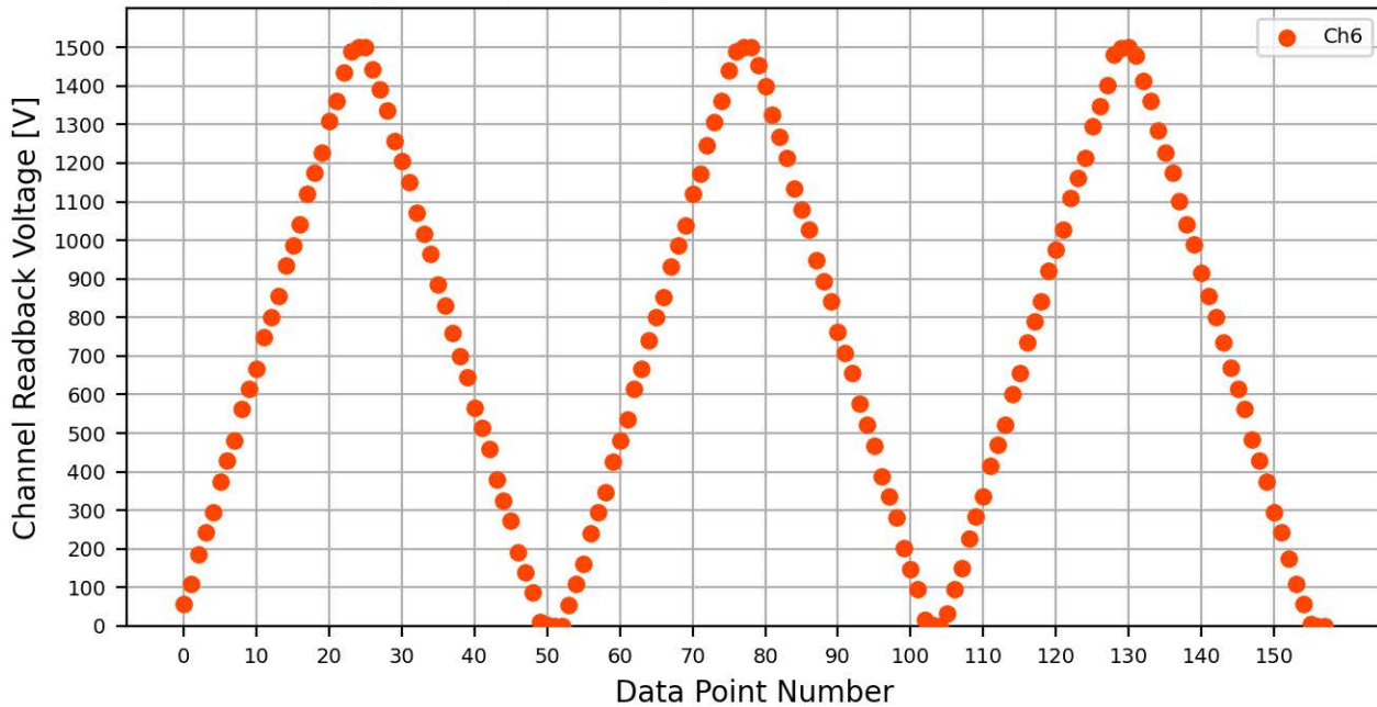
Voltage Ramp Test (Python) Bd #556, Slot #7, Ch #6
