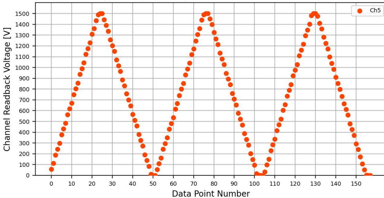
Voltage Ramp Test (Python) Bd #556, Slot #7, Ch #5
