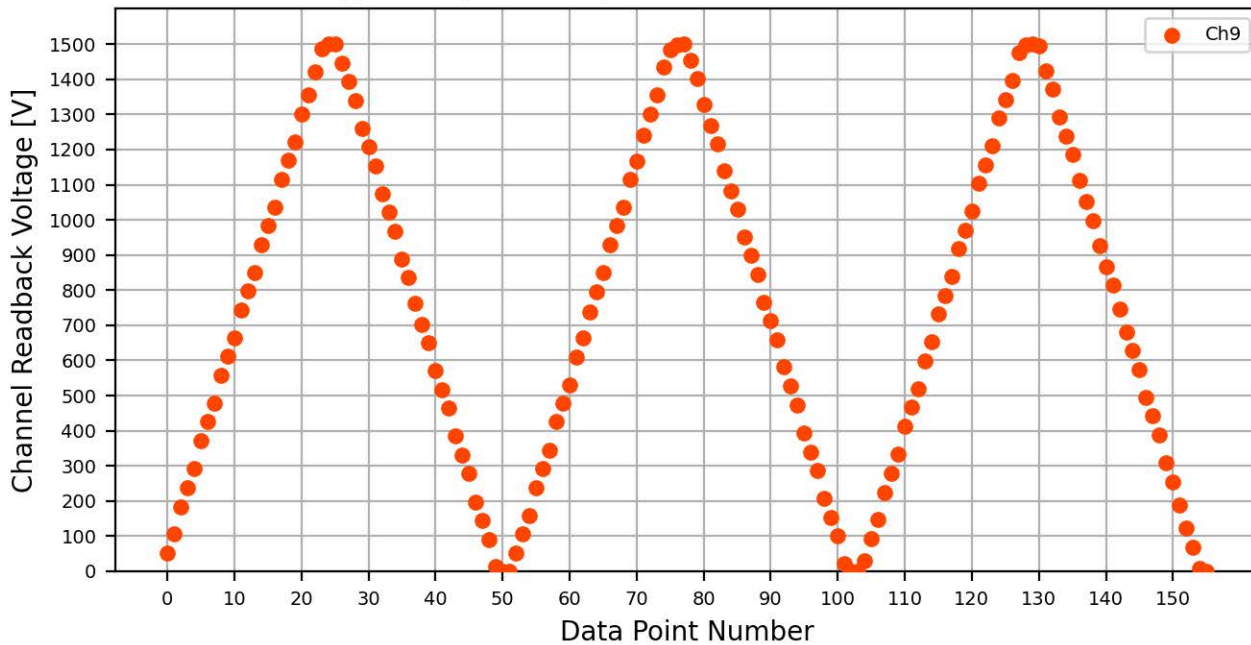
Voltage Ramp Test (Python) Bd #556, Slot #7, Ch #9
