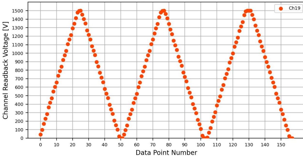
Voltage Ramp Test (Python) Bd #556, Slot #7, Ch #19
