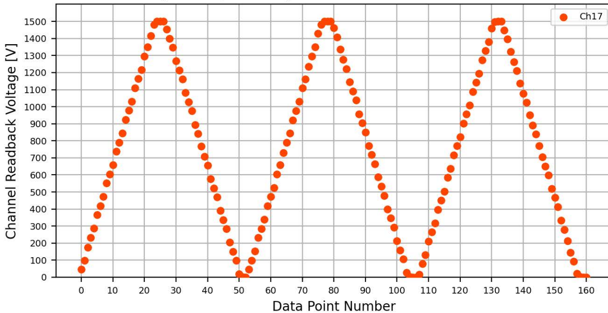
Voltage Ramp Test (Python) Bd #556, Slot #7, Ch #17
