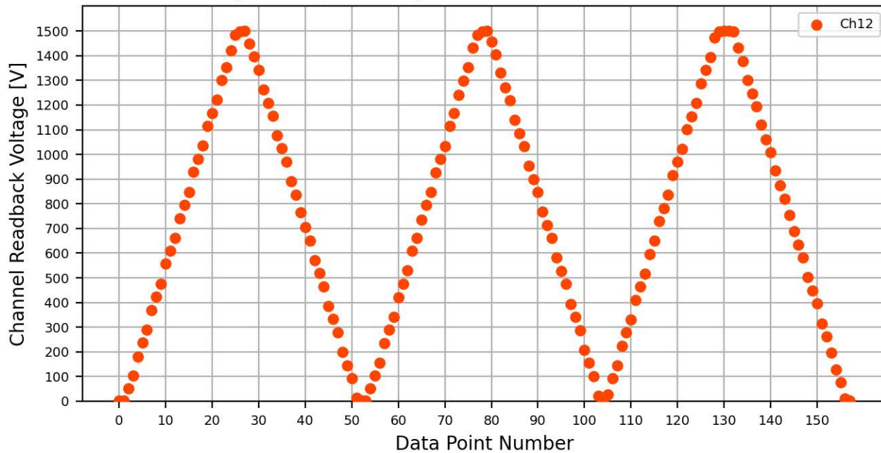
Voltage Ramp Test (Python) Bd #556, Slot #7, Ch #12
