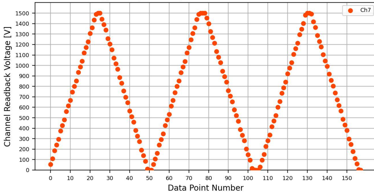
Voltage Ramp Test (Python) Bd #556, Slot #7, Ch #7
