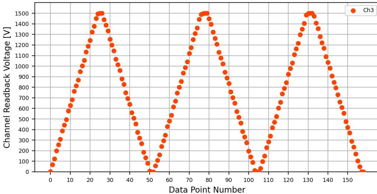
Voltage Ramp Test (Python) Bd #556, Slot #7, Ch #3
