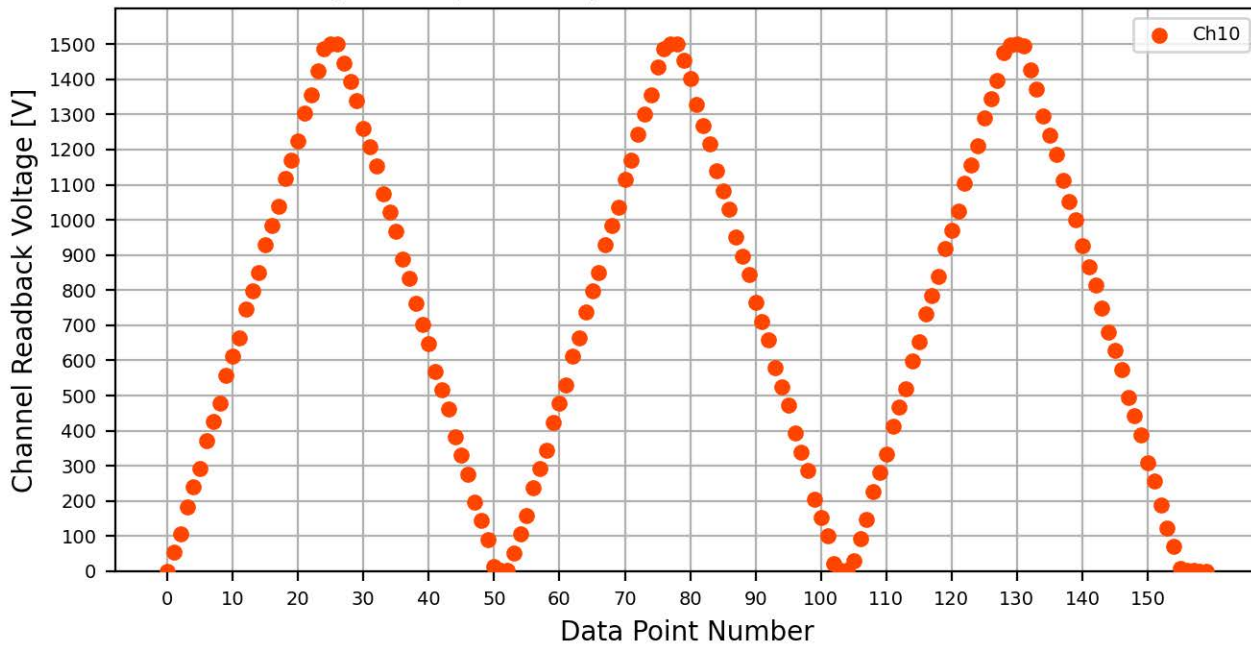
Voltage Ramp Test (Python) Bd #556, Slot #7, Ch #10
