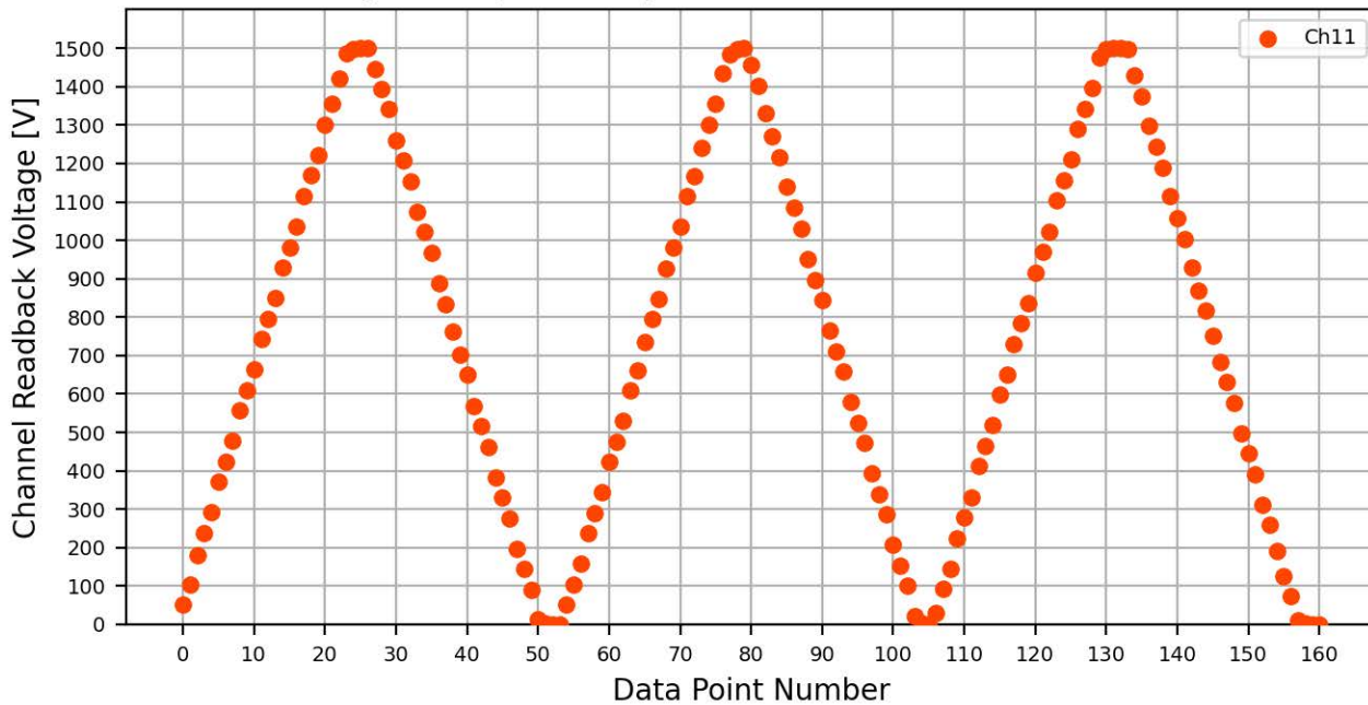
Voltage Ramp Test (Python) Bd #556, Slot #7, Ch #11
