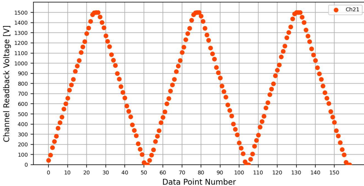
Voltage Ramp Test (Python) Bd #556, Slot #7, Ch #21
