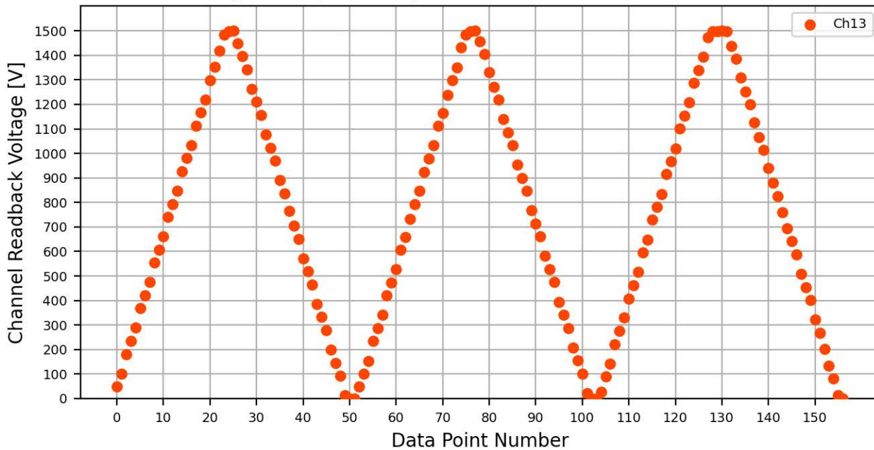
Voltage Ramp Test (Python) Bd #556, Slot #7, Ch #13
