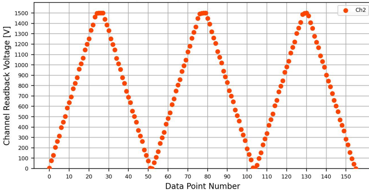
Voltage Ramp Test (Python) Bd #556, Slot #7, Ch #2
