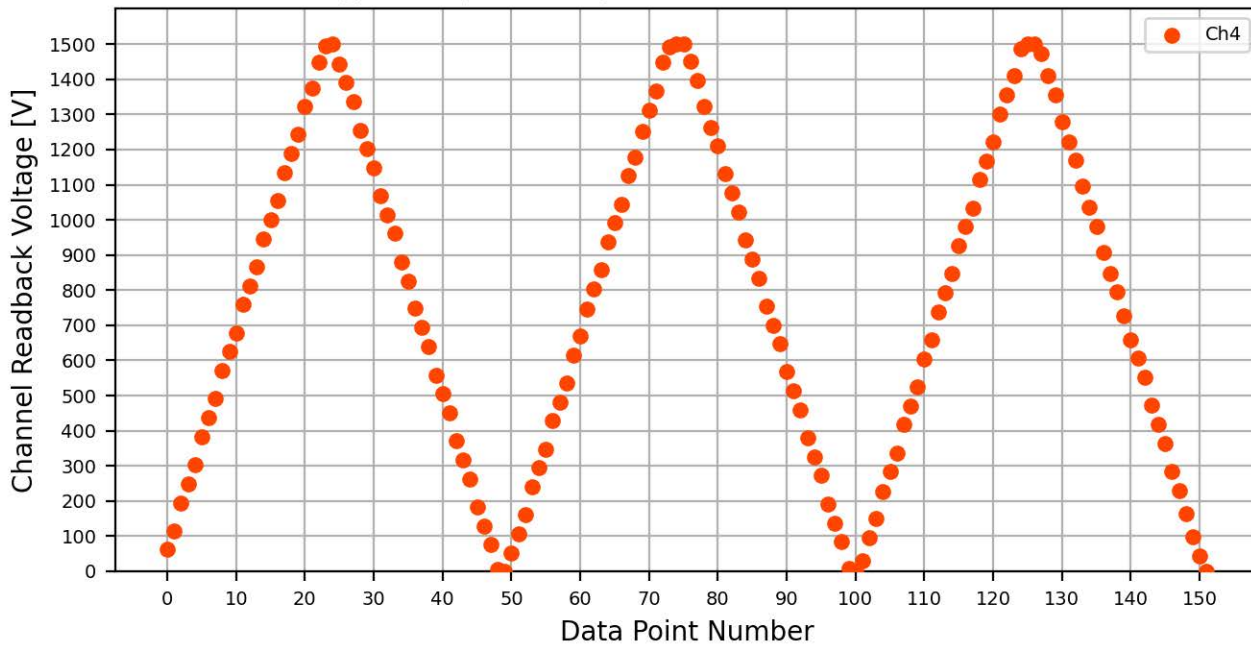
Voltage Ramp Test (Python) Bd #556, Slot #7, Ch #4
