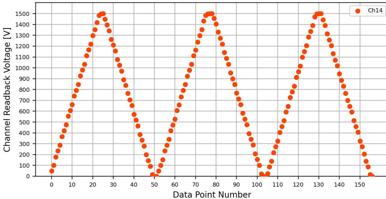
Voltage Ramp Test (Python) Bd #556, Slot #7, Ch #14
