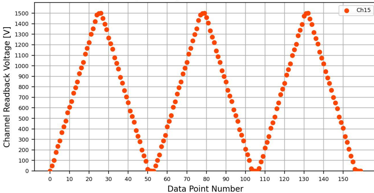
Voltage Ramp Test (Python) Bd #556, Slot #7, Ch #15
