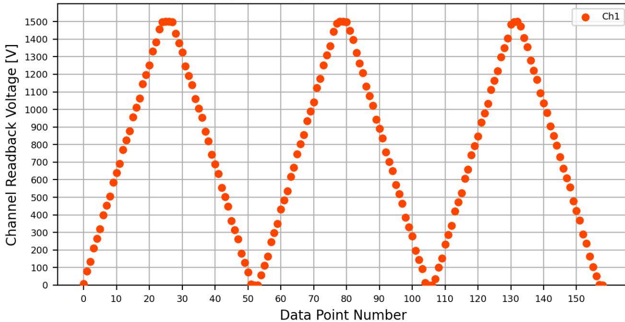
Voltage Ramp Test (Python) Bd #556, Slot #7, Ch #1
