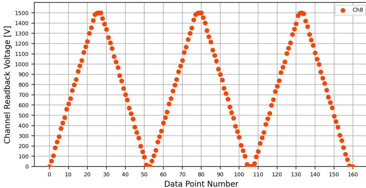
Voltage Ramp Test (Python) Bd #556, Slot #7, Ch #8
