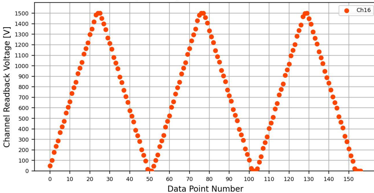
Voltage Ramp Test (Python) Bd #556, Slot #7, Ch #16
