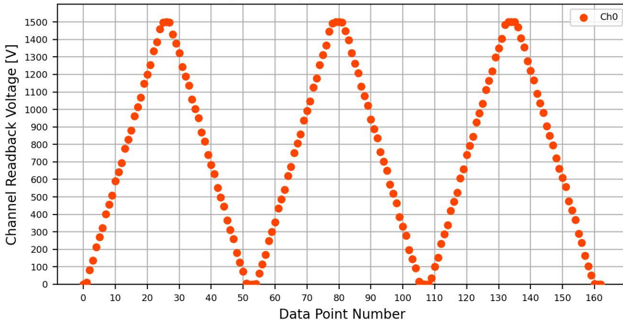
Voltage Ramp Test (Python) Bd #556, Slot #7, Ch #0
